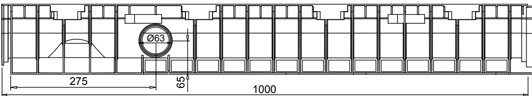
FRONT VIEW
