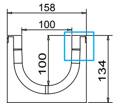
LATERAL VIEW
