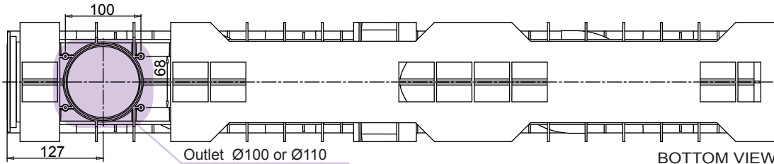
BOTTOM VIEW
