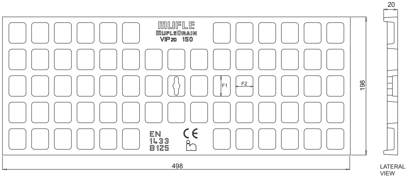
TOP VIEW
