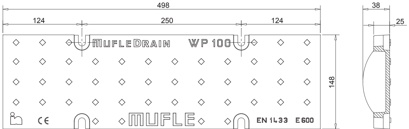
TOP VIEW
