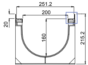
DETAIL FRONT VIEW
