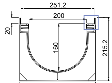
DETAIL FRONT VIEW
