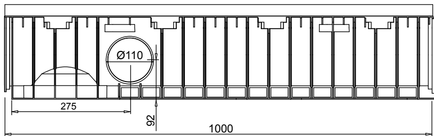
LATERAL VIEW
