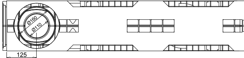
BOTTOM VIEW
