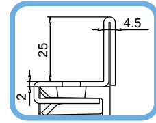
DETAIL SECTION
