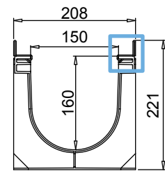
SECTION
