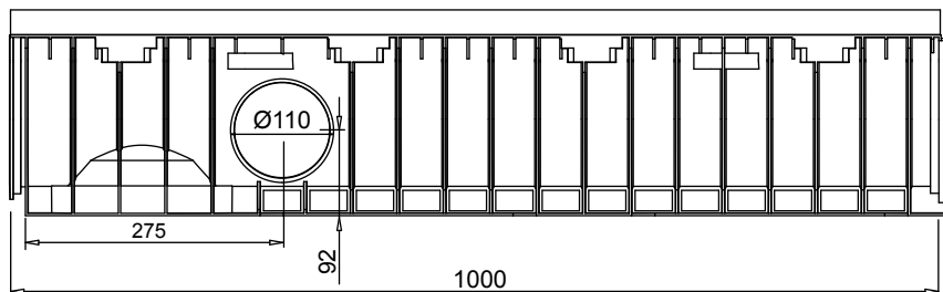
LATERAL VIEW
