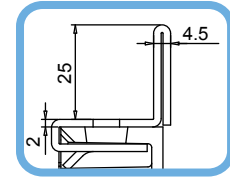
DETAIL SECTION
